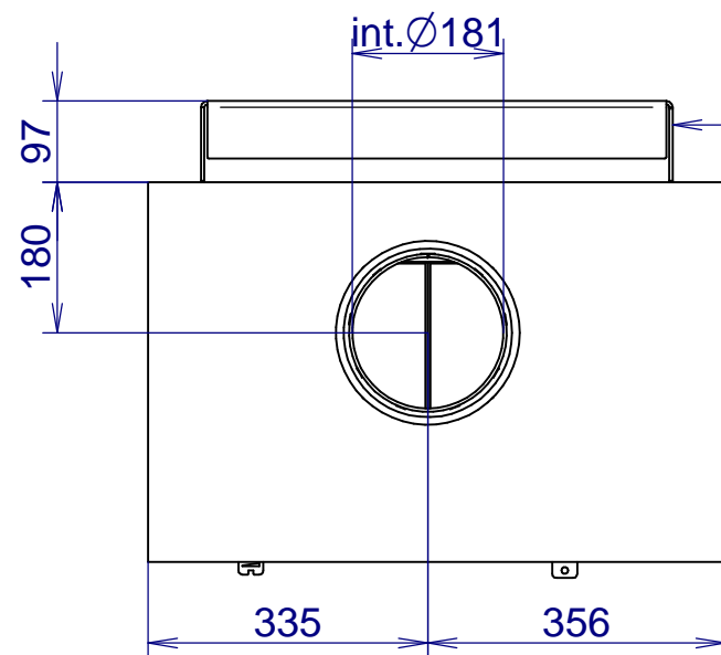
VENUS 630 CL V23 in the box + console for wall
